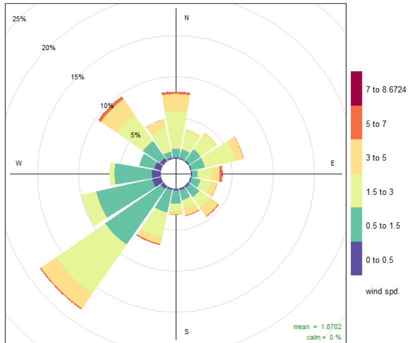
Figure A12: Frequency of (10-minute) wind direction (from) and wind speed measured at Whareroa Marae; 1 Jan – 31 Dec 2021
