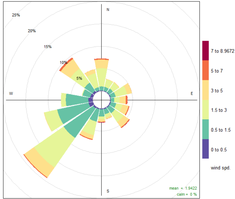
Figure A11: Frequency of (10-minute) wind direction (from) and wind speed measured at Whareroa Marae; 1 Jan – 31 Dec 2020
