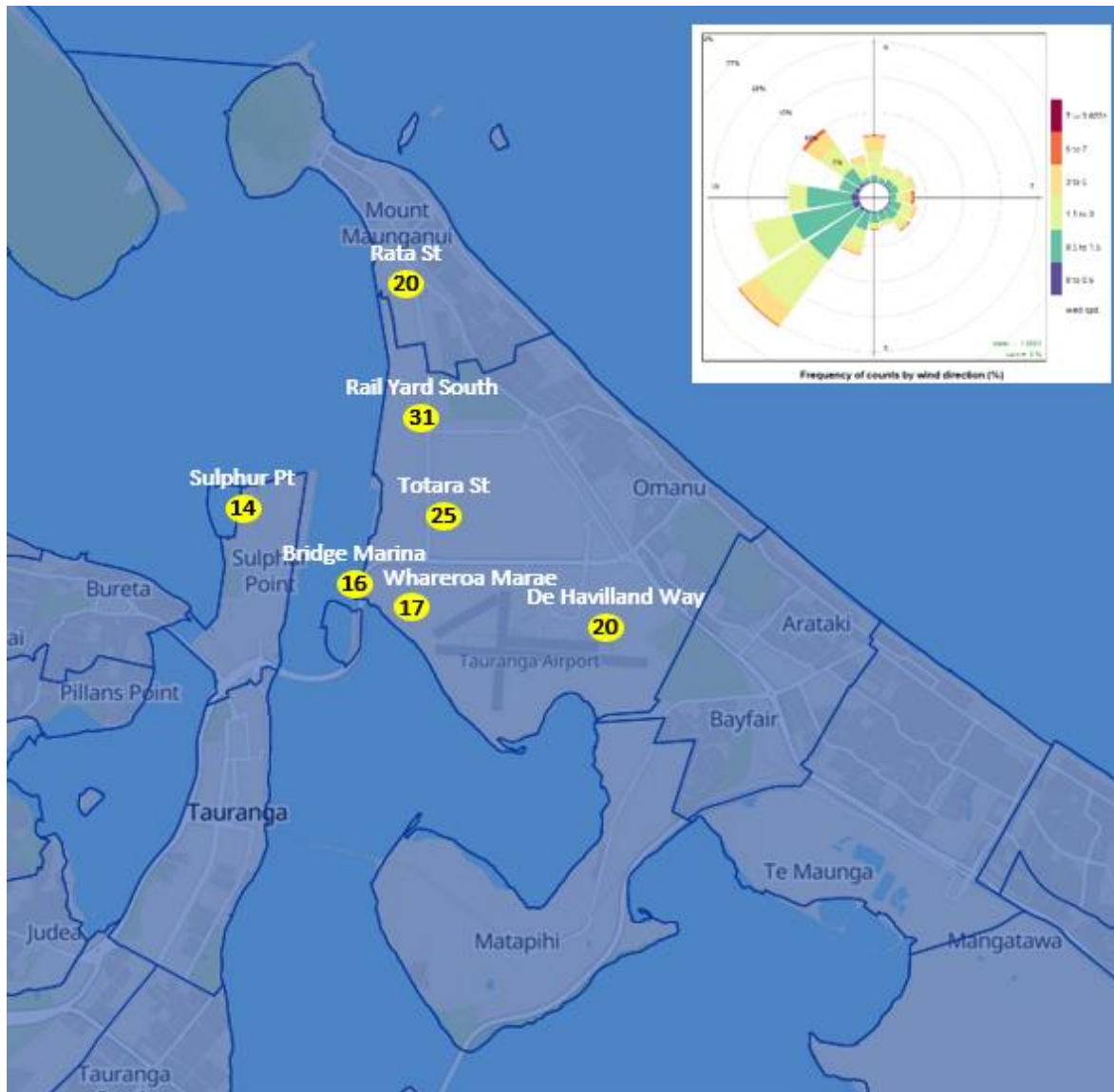
FIGURE 8: 2019 PM 10 monitoring locations and annual PM 10 concentrations measured in the Mount Maunganui Airshed [Source: BOPRC. Insert 2019 wind rose from Whareroa Marae (refer Fig A10)]
